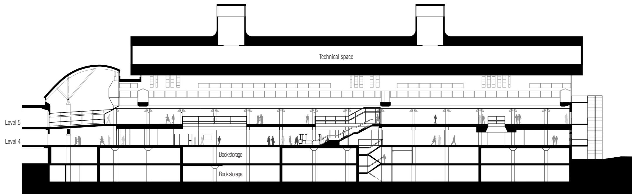
Section AA 1:400
